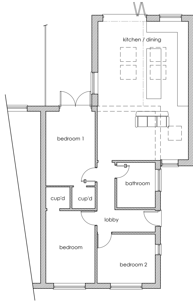
ground
