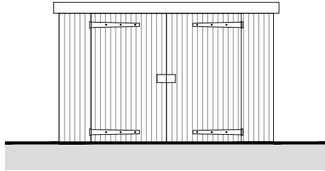
1. Proposed Front Elevation 1:50 @ A4
