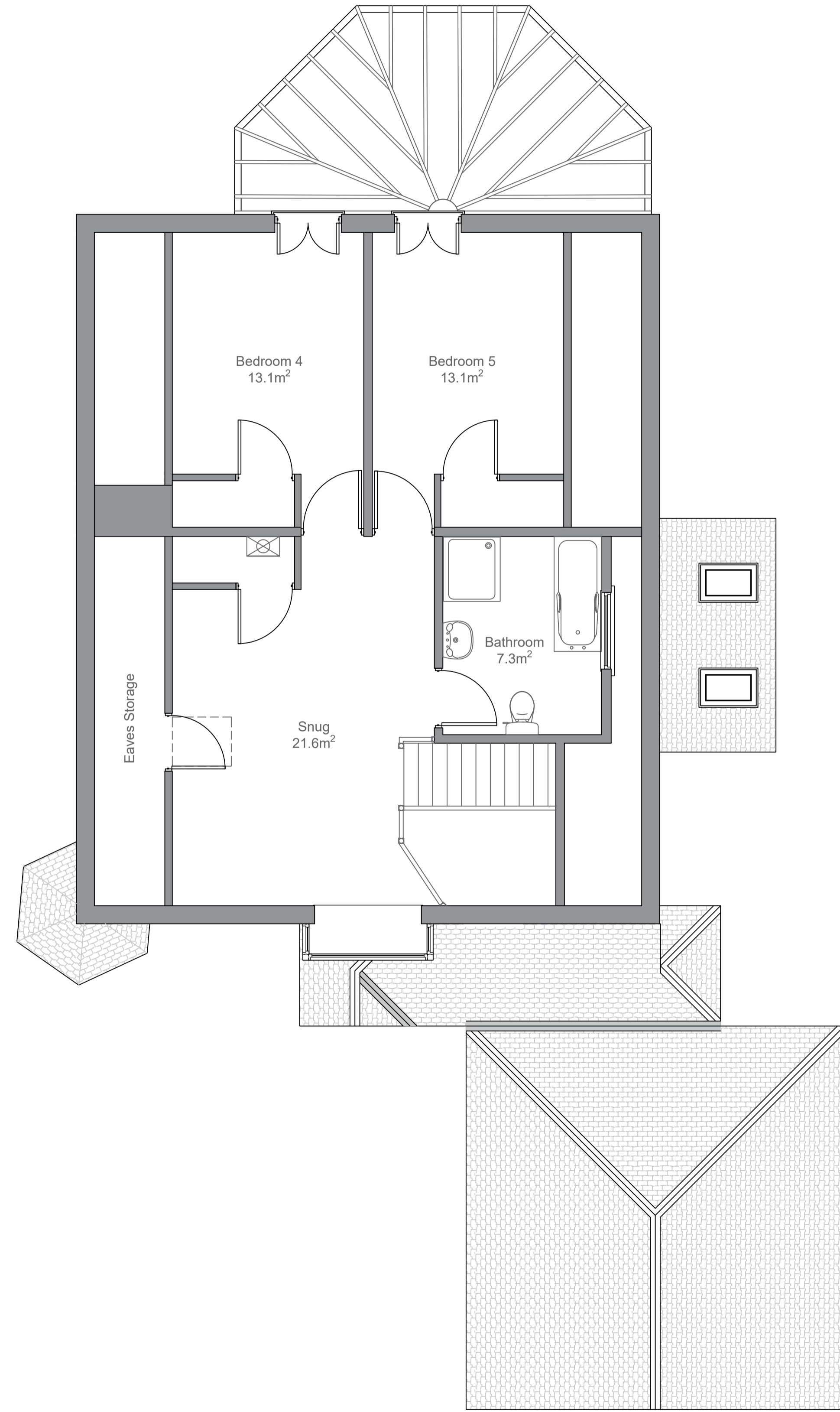
Second Floor 1:50
