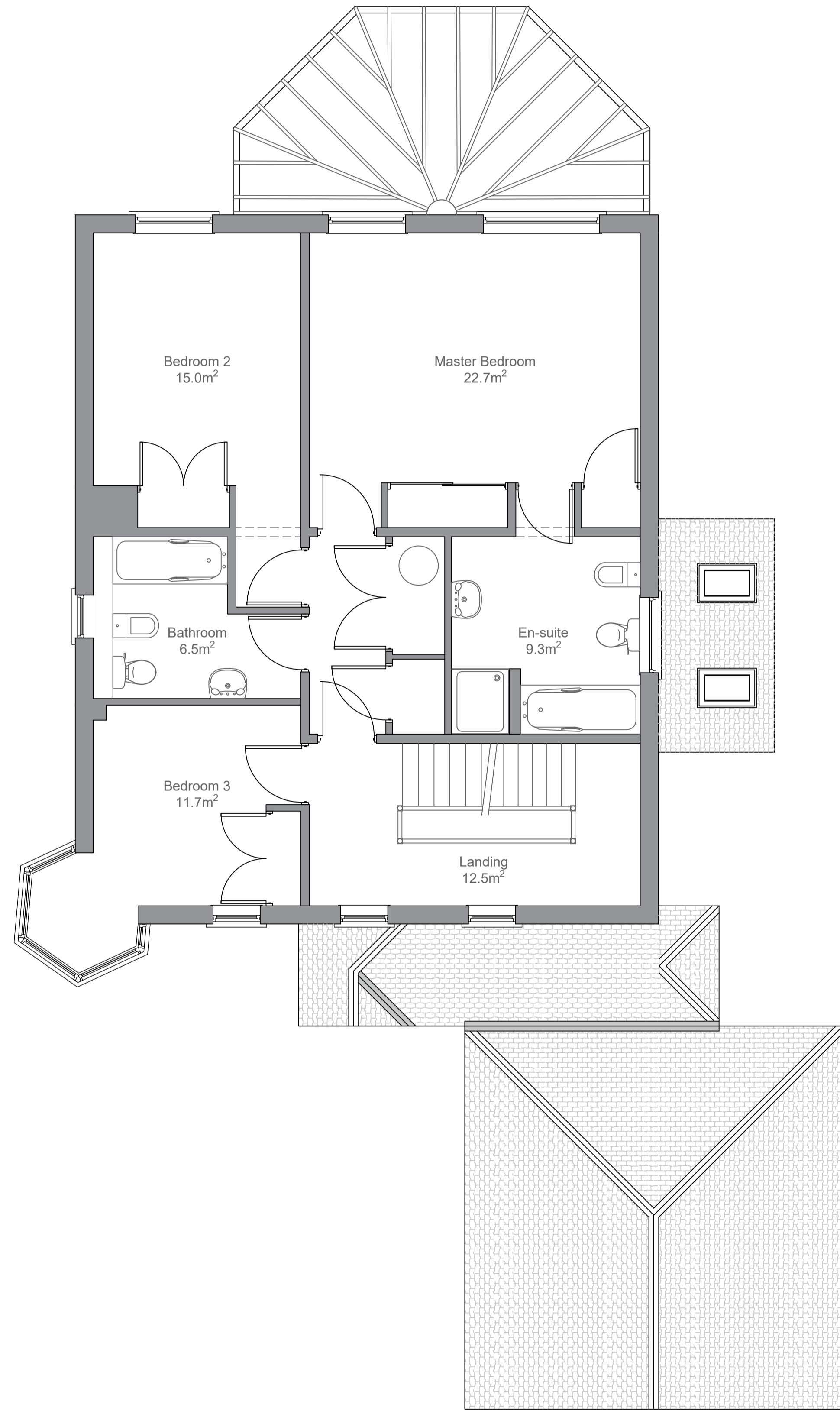
First Floor 1:50
