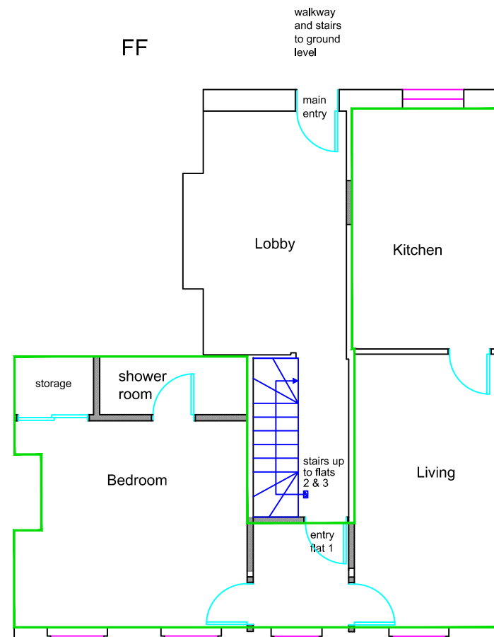
Flat 1 Area = 49.93m 2
