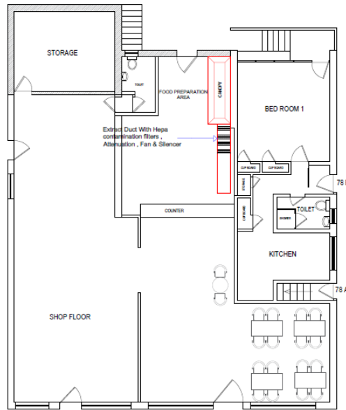
Figure 3 : Proposed Ground Floor Plan
