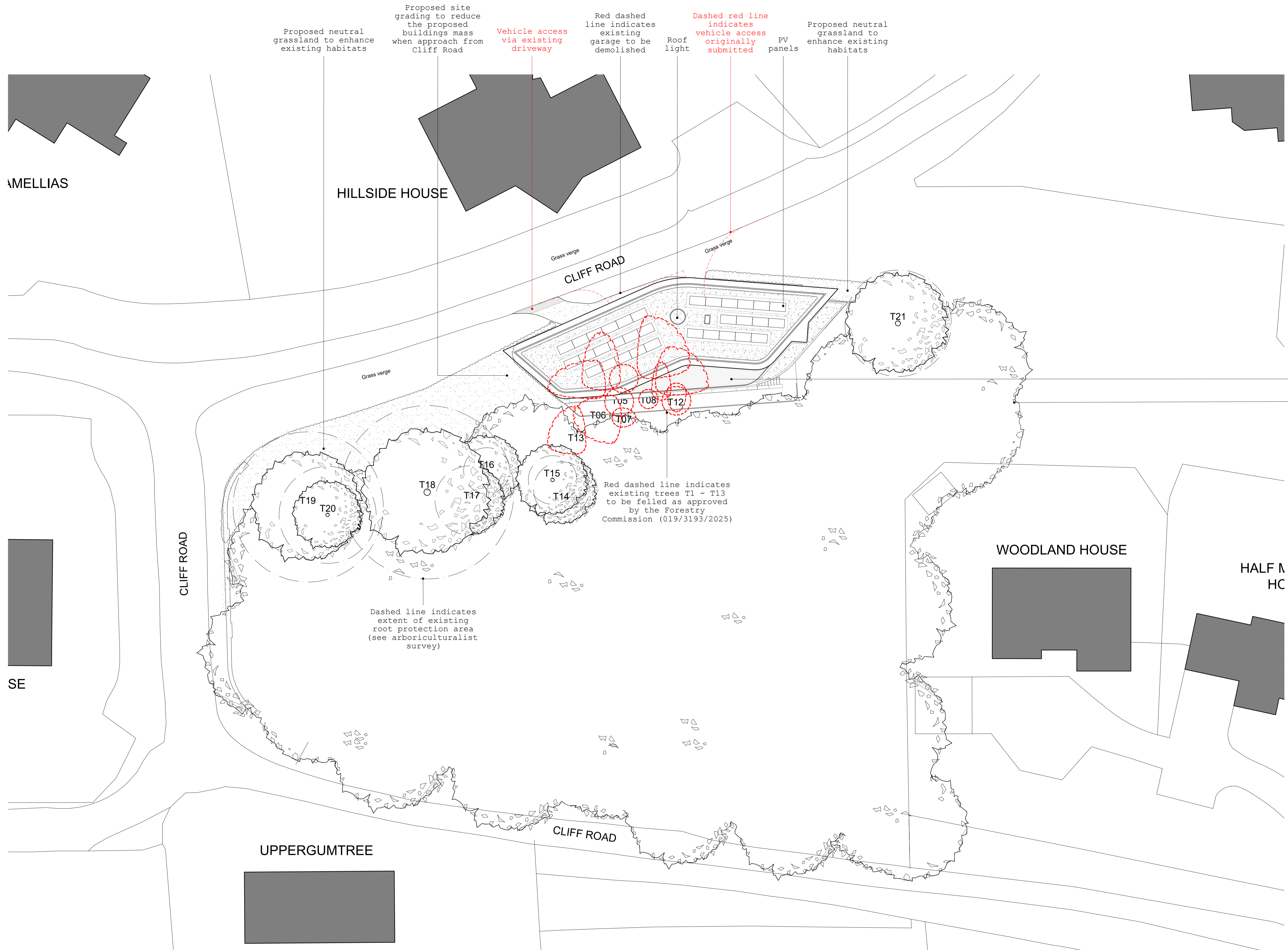
PROPOSED ROOF MASTERPLAN 1:200 @ A1
